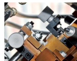
中爪調整機構 The middle pincer adjustment structure
