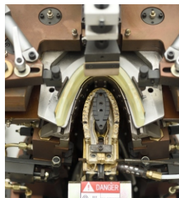
胶盘、扫刀、束紧器、一二爪根据 客户楦头订制 Injector, wiper, toe band, first and second pincers making according customers shoelasts.
