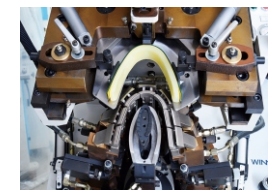
控台、爪子機械 Last supporter and pincers mechanism
